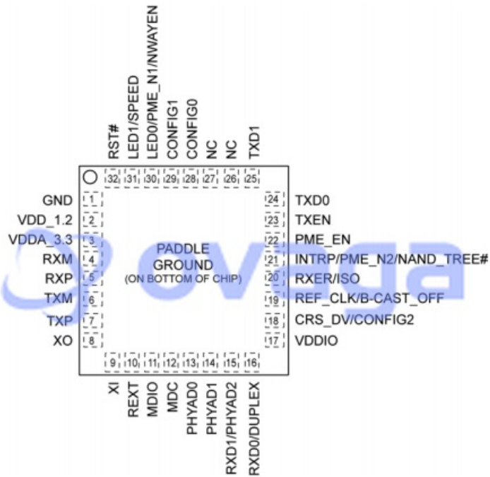
32-Pin (5mm × 5mm) QFN
