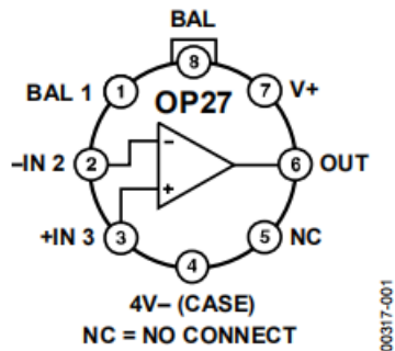
Figure 1. 8-Lead TO-99 (J-Suffix)
