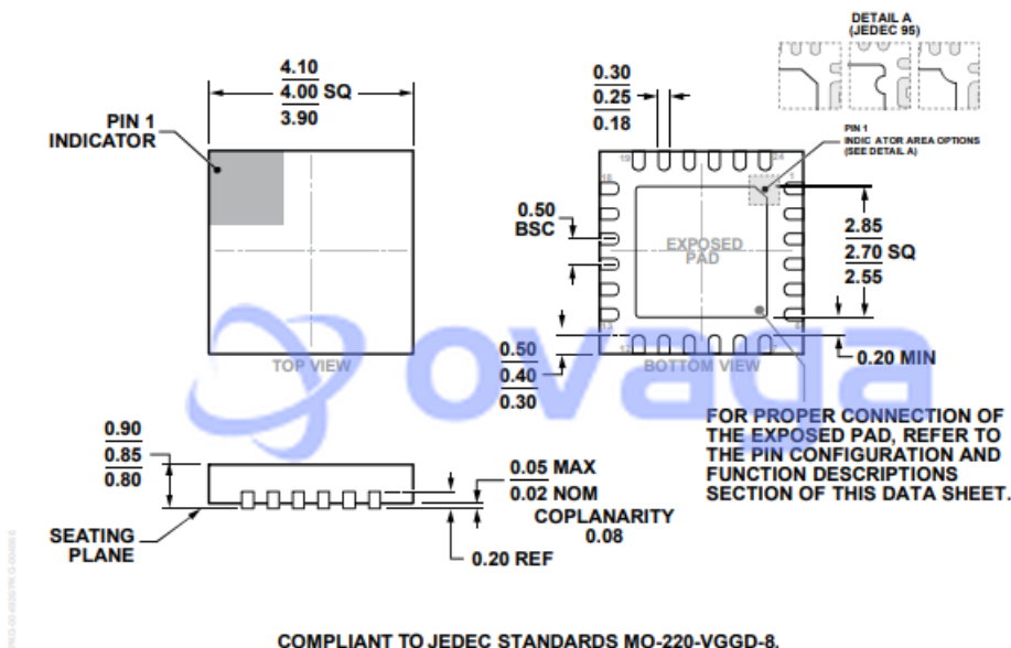
Figure 28. 24-Lead Lead Frame Chip Scale Package [LFCSP] 4 mm \times 4 mm Body and 0.85 mm Package Height (CP-24-16)
